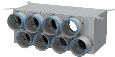
Standard air distribution box 160-12x75 body with 8 flanges
